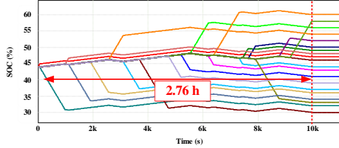
Fig. 4: Time trend of SOC of the cell by the proposed method.
