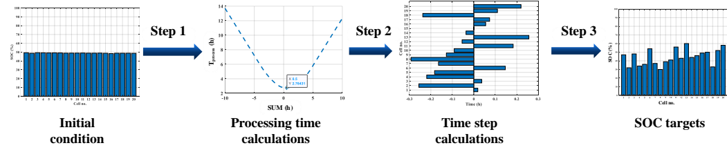
Fig. 3: De-balancing workflow
